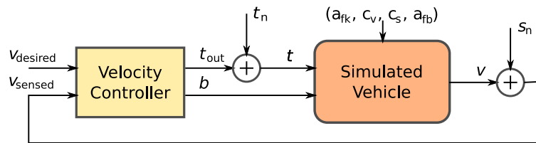
Figure 3: Velocity simulation model.
