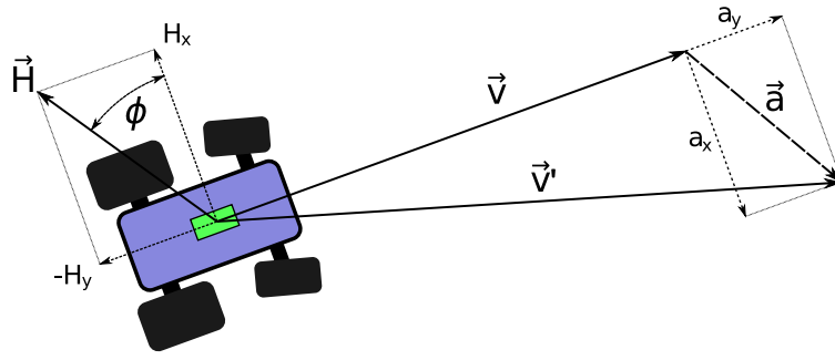
Figure 1: Vehicle vectors.
