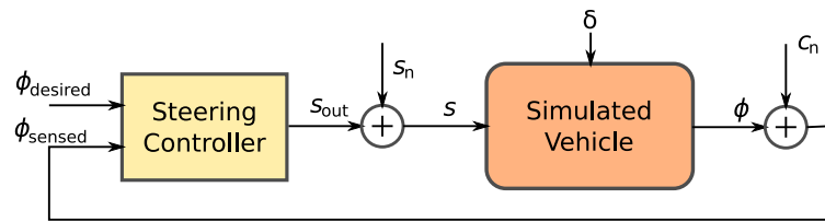
Figure 2: Heading simulation model.
